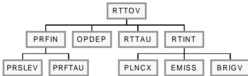
Figure A2. Subroutine tree for RTTOV-5 main call
